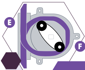
Straight-Thru Design™ eliminates tube destroying pinch points, as seen in the alternate threading patterns below.
